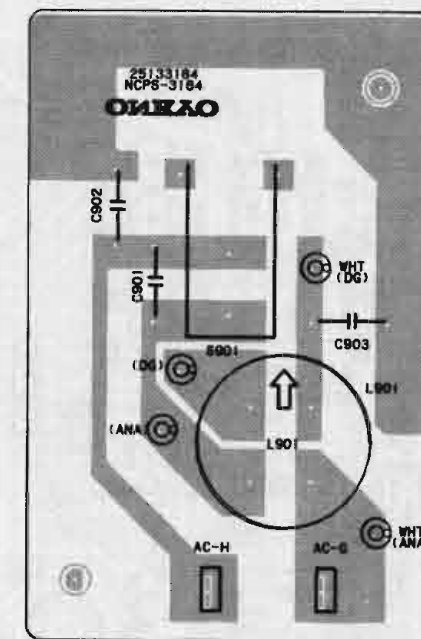
POWER SUPPLY CIRCUIT PC BOARD
