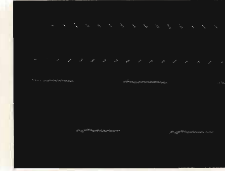
Photo 4 Upper OSC output Pin 3 of Q302 Lower BCLK signal Pin 5 of Q302 Vertical:2V/div. Horizontal:0.1 \mu s/div.
