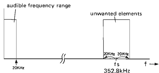
Fig. 15 F_s = 352.8\text{kHz}
