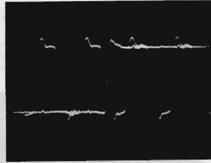
Photo 5 Range:Vertical:1V/div. Horizontal:50nS/div. Synchronize with WCK.
